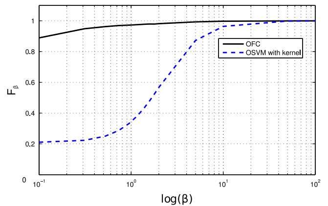
Fig. 6. Algorithm comparison using skin segmentation data. F -measure for OFC (in black) and one class SVM (in blue). (For interpretation of the references to color in this figure caption, the reader is referred to the web version of this article.)
