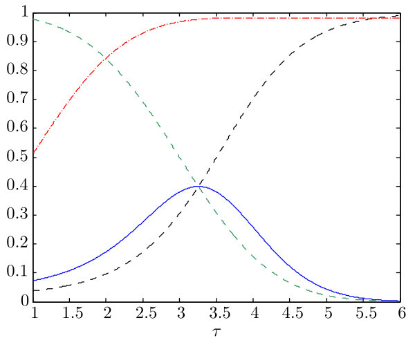
Fig. 3. Performance measures for several values of the decision threshold \tau , for the unidimensional problem with \beta = 1 . F -measure in blue (solid), Recall in green (decreasing dashed), Precision in black (increasing dashed) and Accuracy in red (dash-dot). (For interpretation of the references to color in this figure caption, the reader is referred to the web version of this article.)
