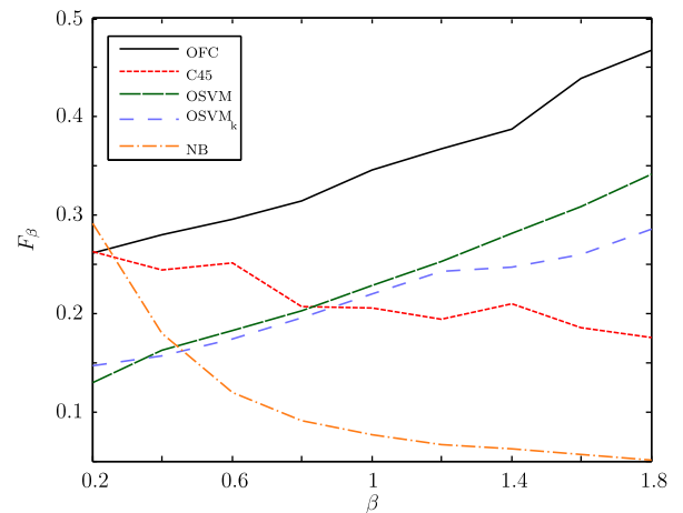
Fig. 5. F_\beta performance of the different classifiers, for several values of \beta .
