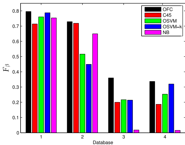
Fig. 4. F_\beta values for different classifiers using databases 1–4.
